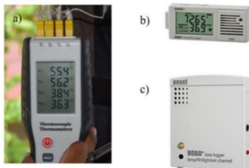
Figure 2. Instruments used (a) Thermocouple Channel Type K HT-9815, Thermocouple temp; (b) Hobo-1, Hobo temp/Relative Humidity (RH); and (c) Hobo-2, Hobo temp/RH/Light/External logger
