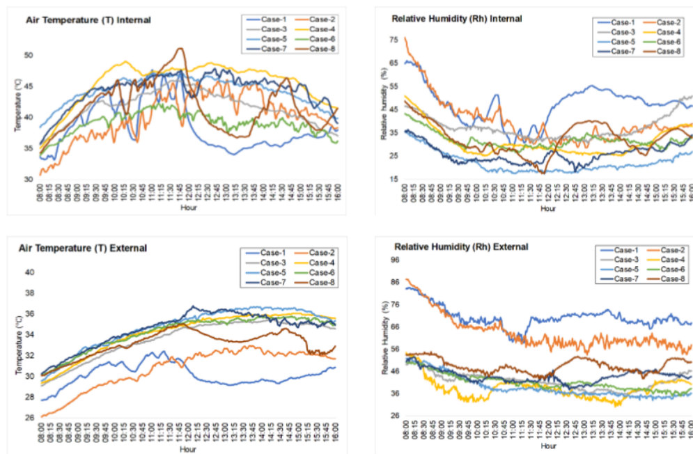
Figure 3. Temperature graph, internal relative humidity and external of attics T-internal = attic temperature, T-external = environment temperature, Rh-internal = attic relative humidity, and Rh-external = environment relative humidity
